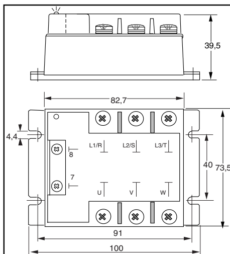
Dimensions / Dimensions:
