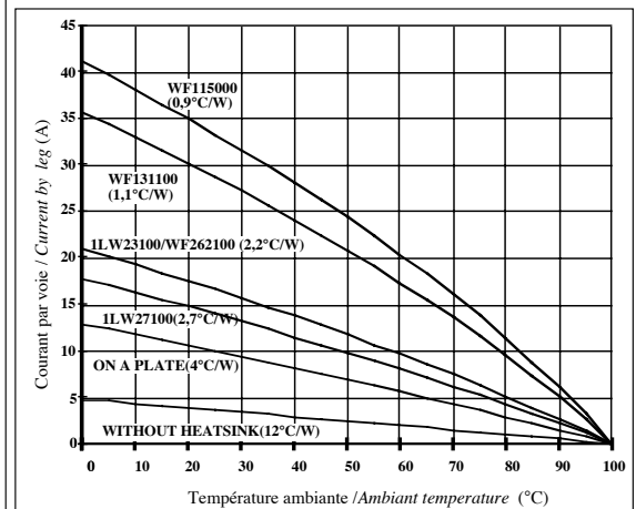
Fig.2 Courbes thermiques /Thermal characteristics
