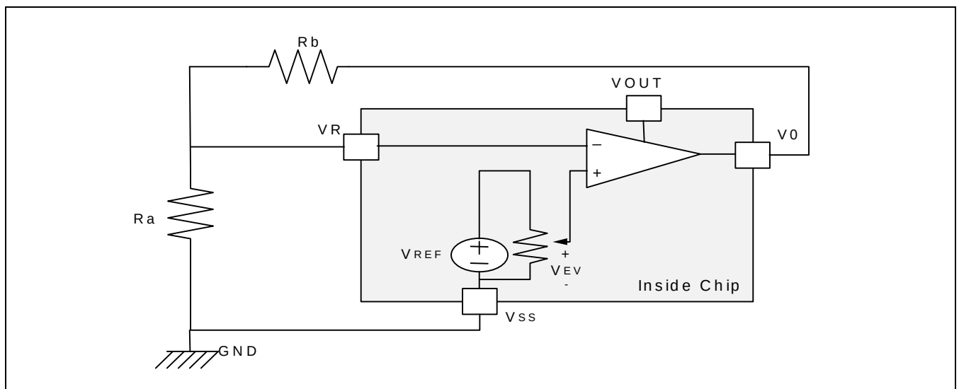
Figure 20. Electronic Contrast Control Circuit
