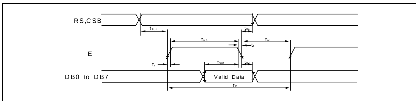
Figure 36. Write Bus Mode Timing Diagram (68 Mode)
