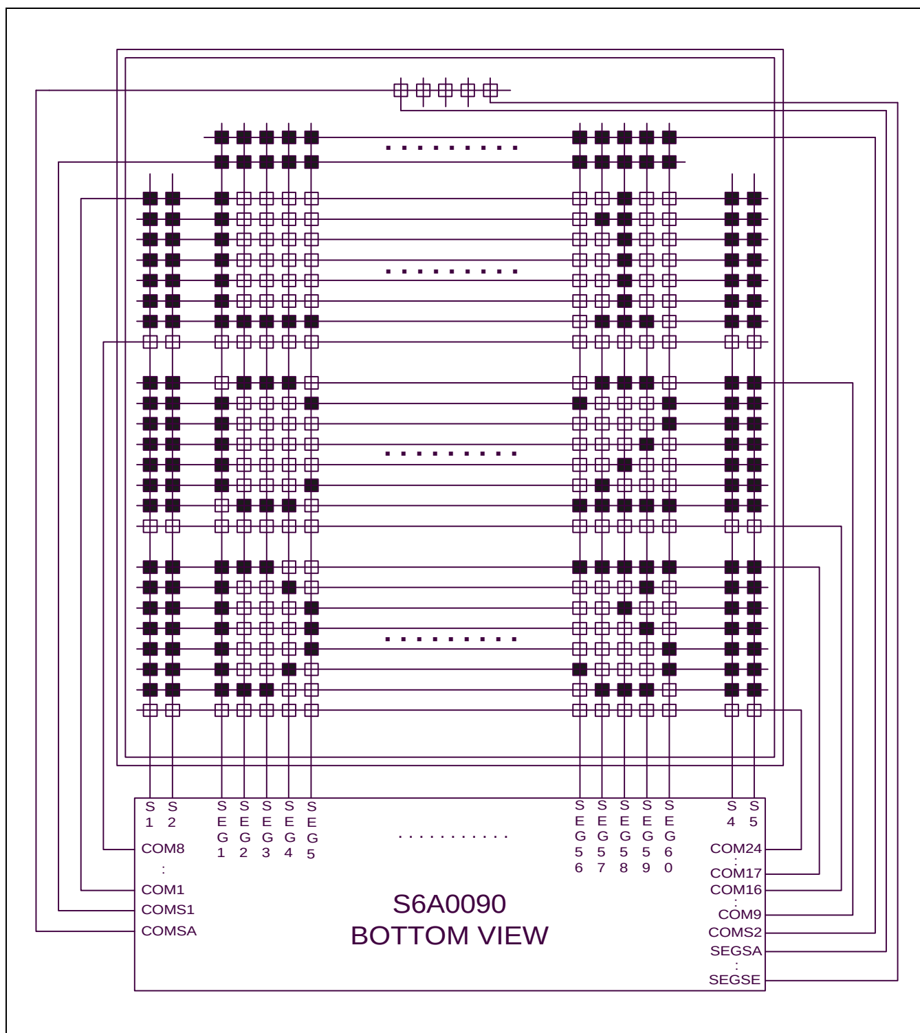
Figure 27. Chip Bottom &amp; Lower View (S (COM) = "0", BID (SEG) = "0")
