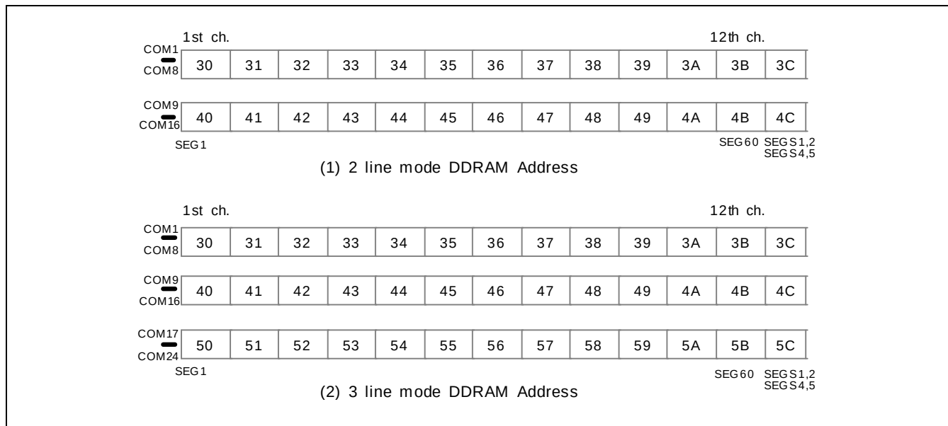
Figure 8. DDRAM Address
