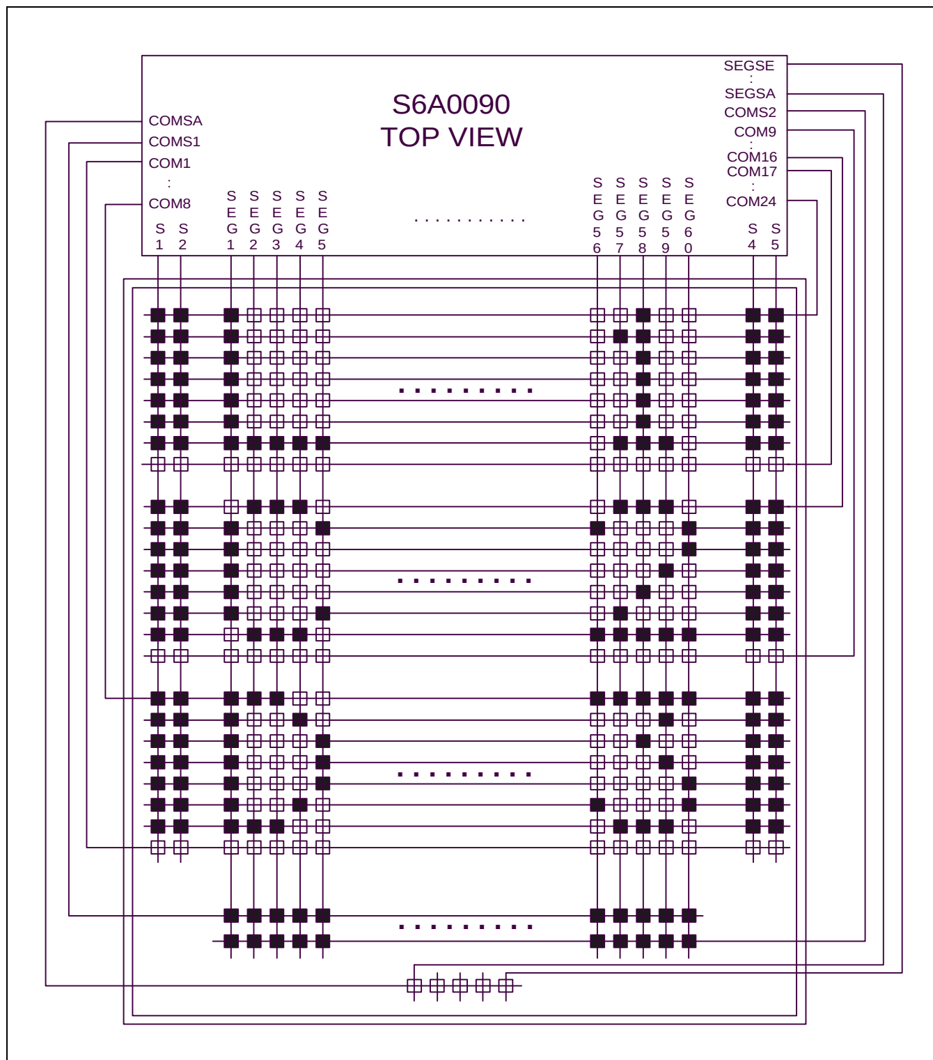
Figure 30. Chip Bottom & Upper View (S (COM) = "1", BID (SEG) = "0")
