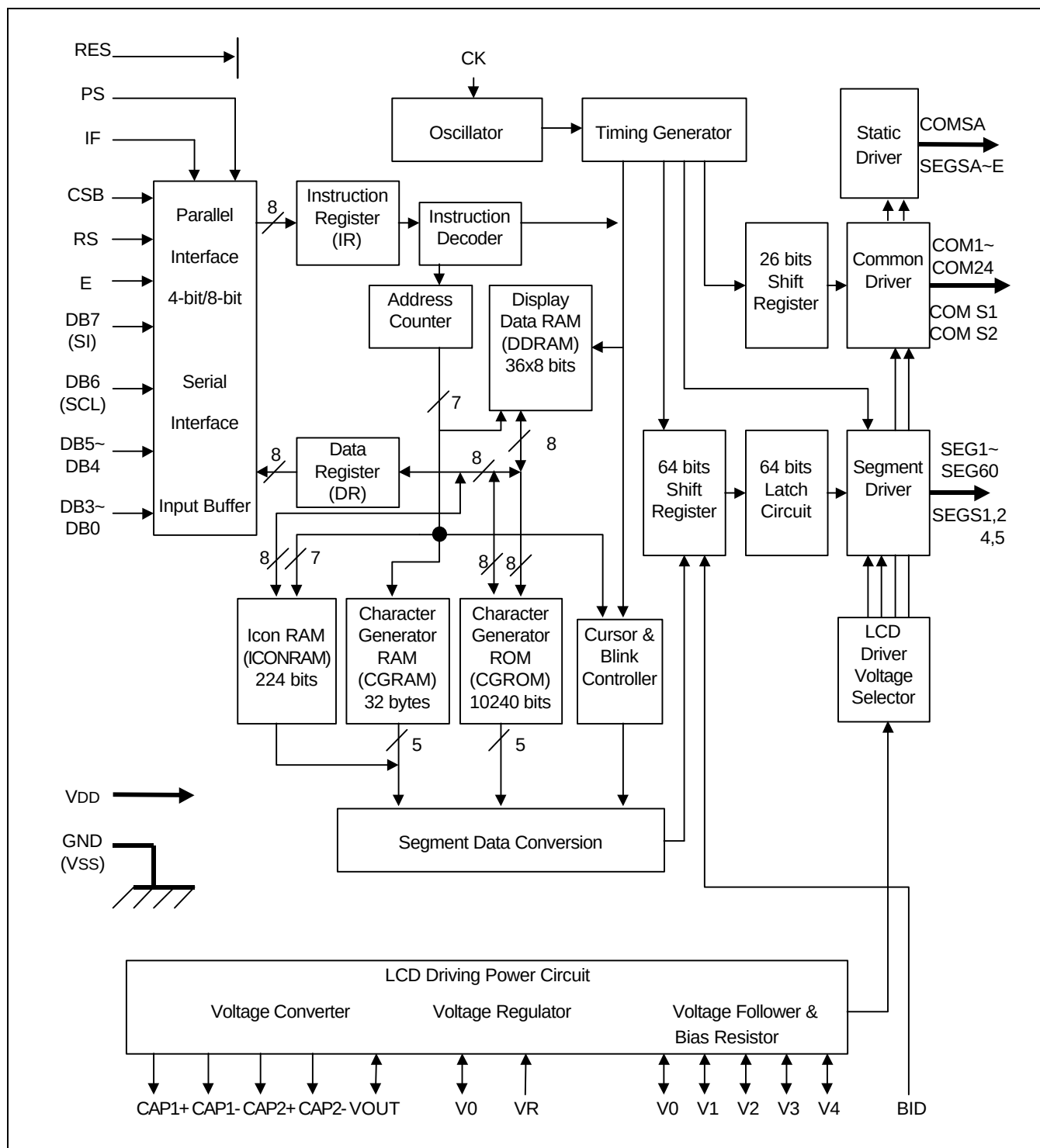
Figure 1. Block Diagram
