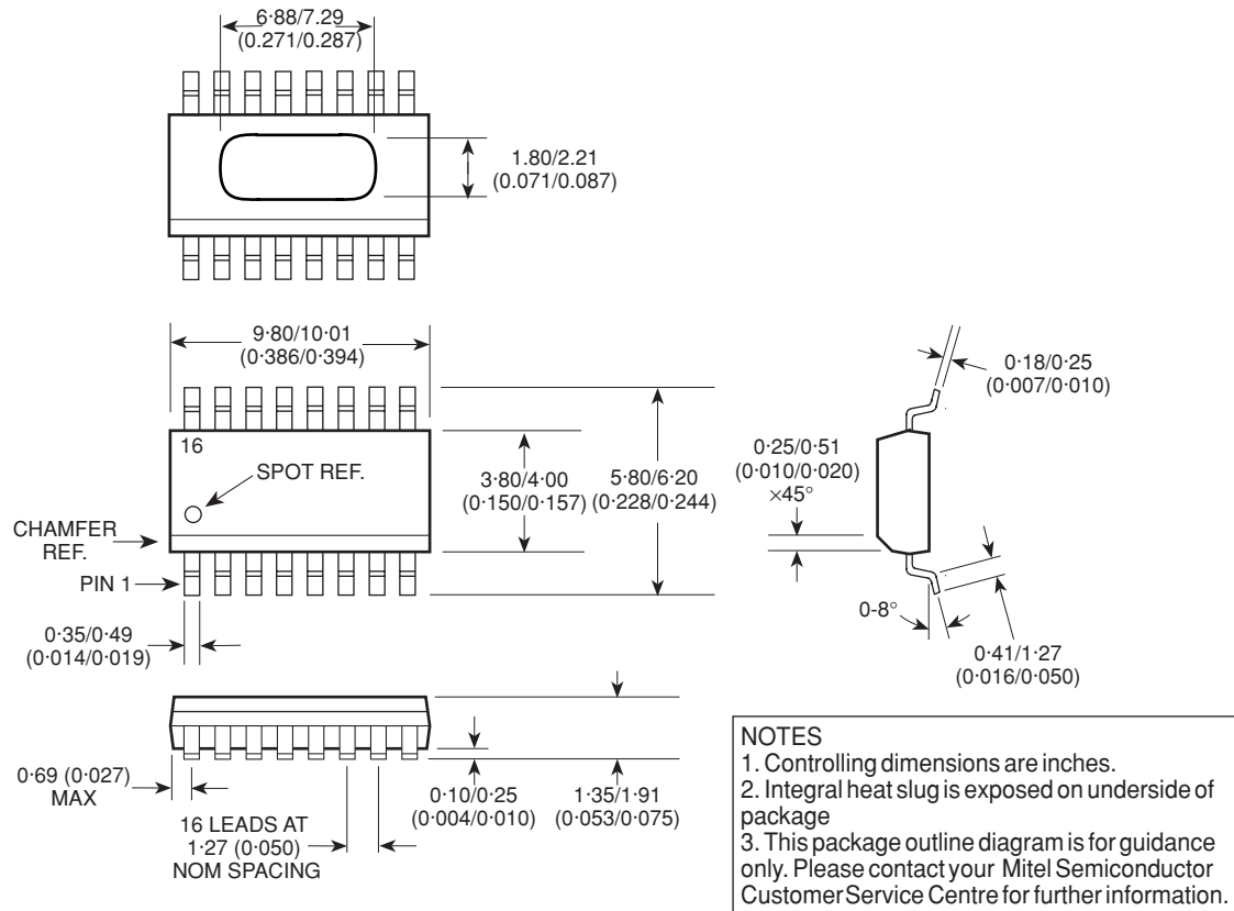
16-LEAD MINIATURE HEAT SUNK PLASTIC DIL - MH16
