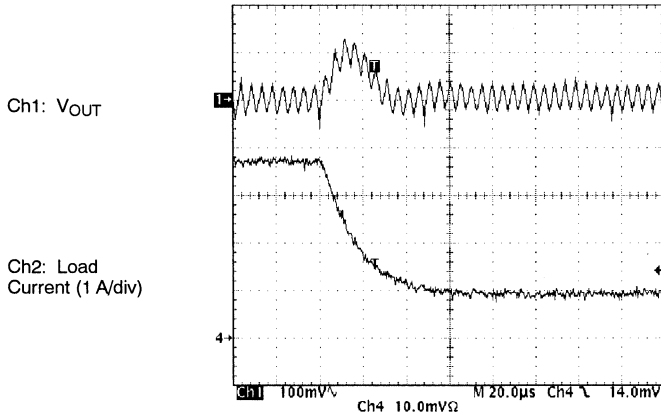
PWM Unloading
