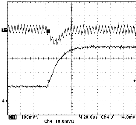
PWM Loading
