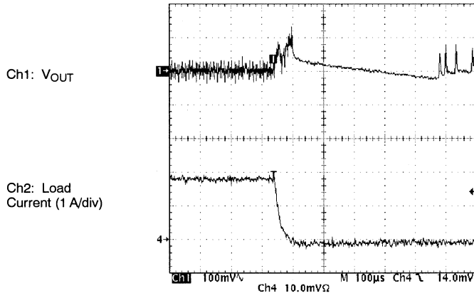
PWM to PSM
