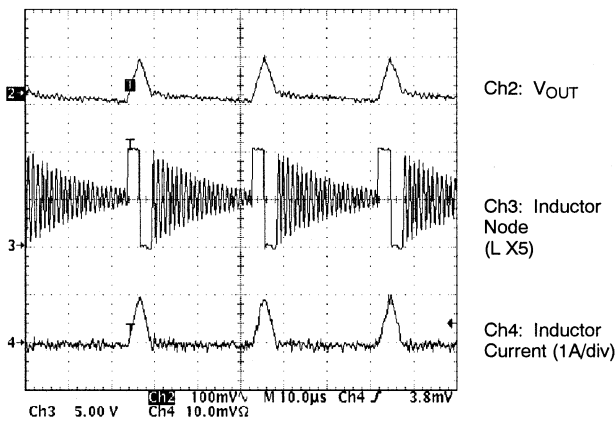
PSM Operation
