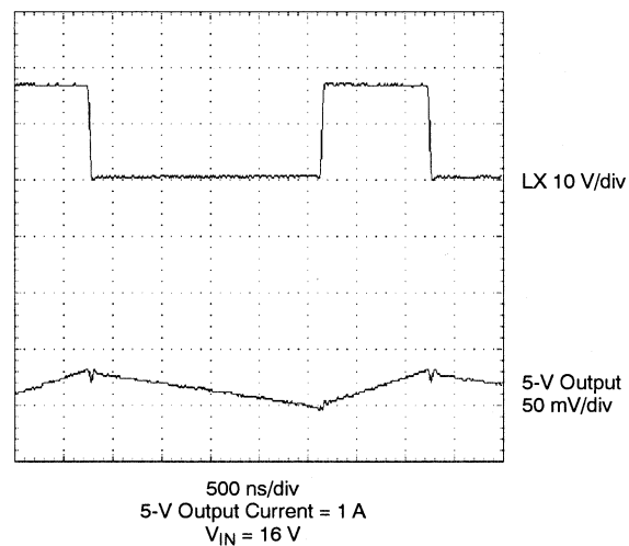
Pulse-Width Modulation Mode Waveforms
