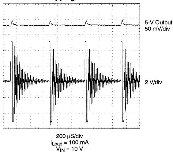
Pulse-Skipping Waveforms
