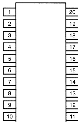
SOIC-20 Wide-Body
