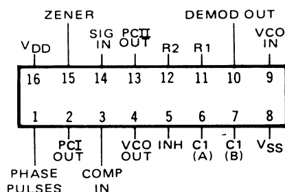
CONNECTION DIAGRAM
