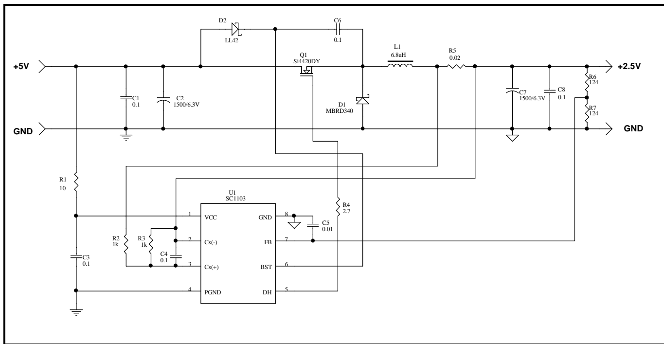
Fig. 9: 5V to 2.5V @ 4A Application with "flying capacitor" boost voltage.
