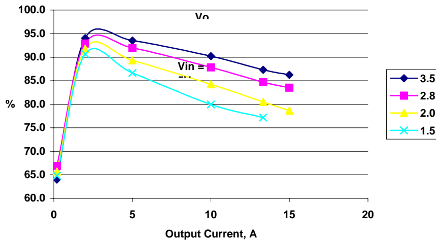
SC1154 Efficiency
