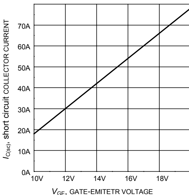
Figure 20. Typical short circuit collector current as a function of gate-emitter voltage ( V_{CE} \leq 400\text{ V} , T_J \leq 150^\circ\text{C} )
