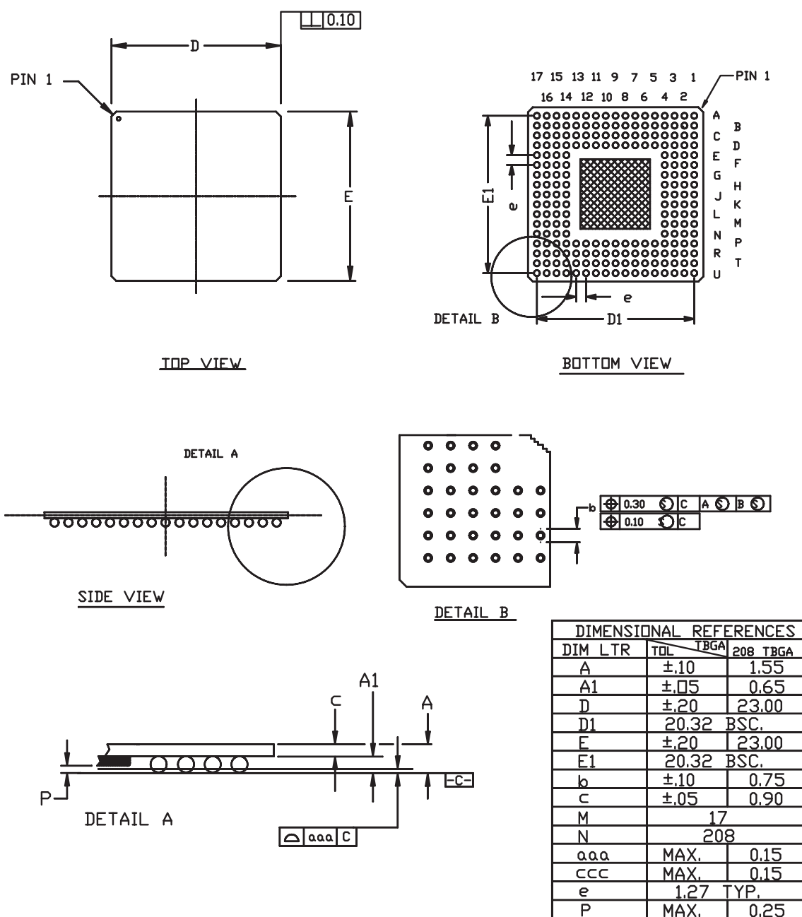
Figure 14. Compact 23mm x 23mm 208 TBGA Package
