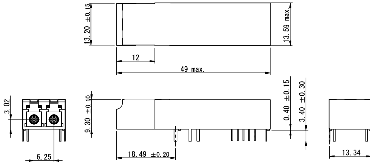
Figure 3. Outline Dimensions (SCM6201-GL-Z#)
