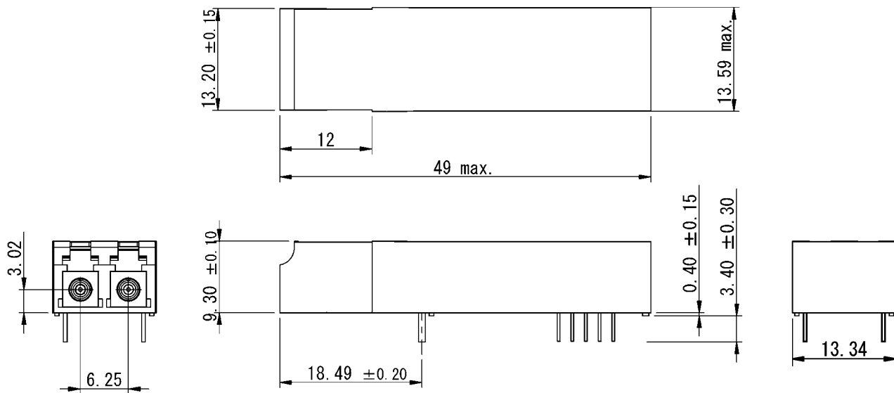
Figure 6. Outline Dimensions (SCM6201-JL-Z#)
