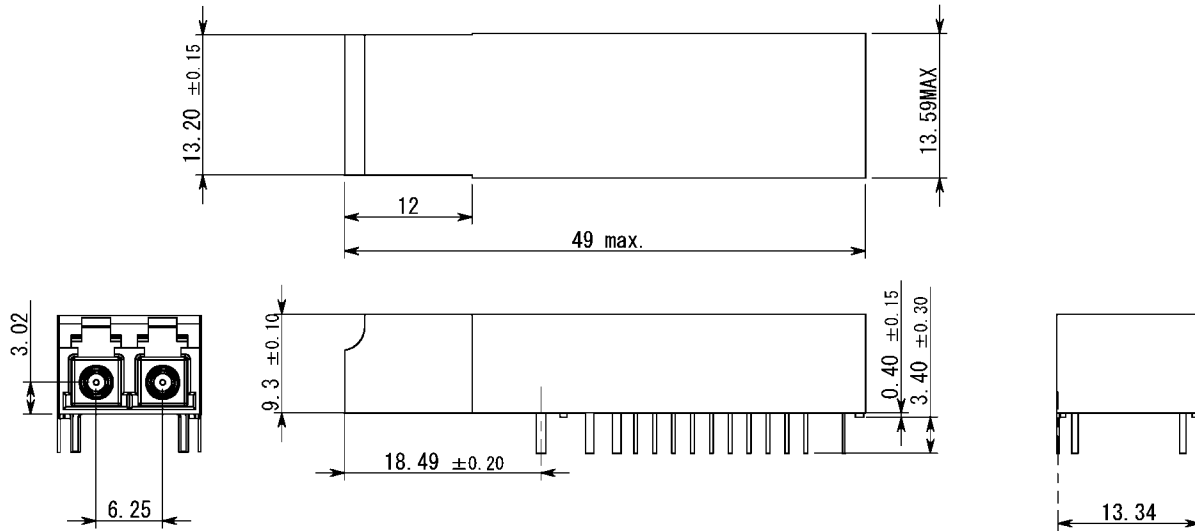
Figure 3. Outline Dimensions(SCM6002-GL-Z#)
