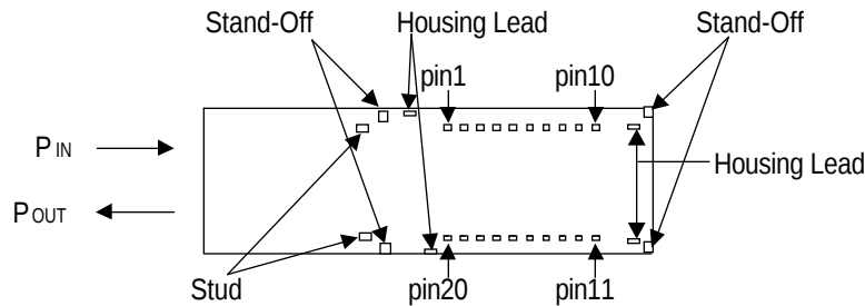
Figure 12. Bottom View
