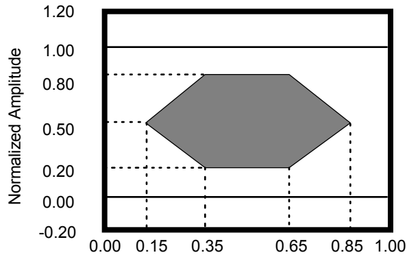
Figure 15. Optical Pulse Mask with Fourth Order
