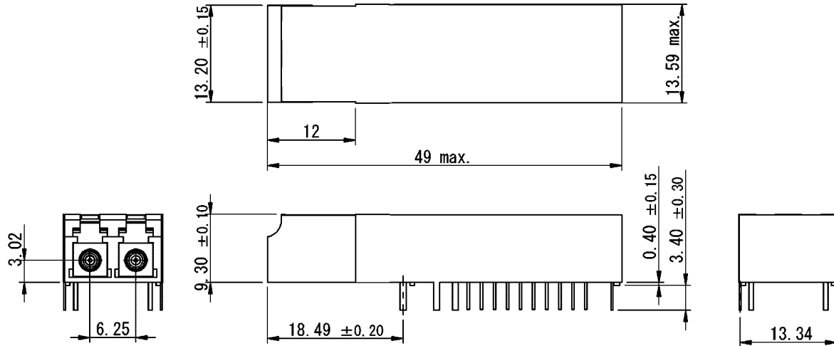
Figure 3. Outline Dimensions(SCM6011-GL-Z#)
