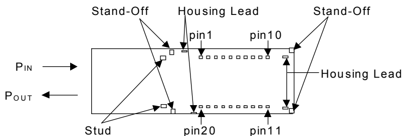
Figure 12. Bottom View
