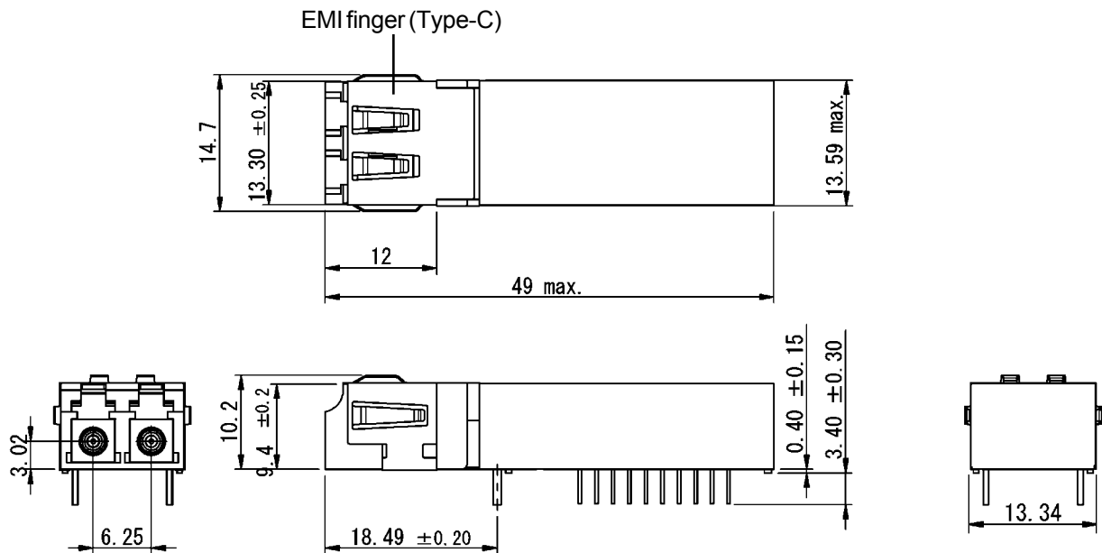
Figure 6. Outline Dimensions (SCM6011-JL-Z#)
