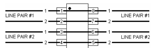
Figure 4A DIFFERENTIAL MODE CONFIGURATION CIRCUIT BOARD LAYOUT
