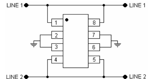
Figure 3 COMMON MODE CONFIGURATION
