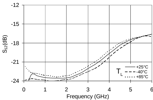
S_{12} vs. Frequency V_D = 3.3 \text{ V} , I_D = 60 \text{ mA} (Typ.)
