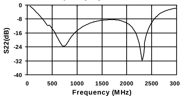
S22 vs. Frequency, I_d = 130 mA, T = +25^\circ\text{C}
