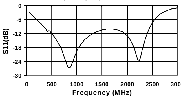
S11 vs. Frequency, I_d = 130 mA, T = +25^\circ\text{C}
