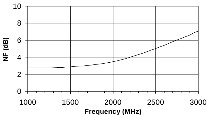
Noise Figure vs. Frequency for SGA-7489 2GHz Tuned Circuit, I_d=130 mA, T=+25^\circ\text{C}
