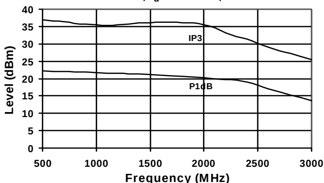
P1dB & IP3 vs. Frequency for 2GHz Tuned Circuit, I_d = 130 mA, T = +25^\circ\text{C}
