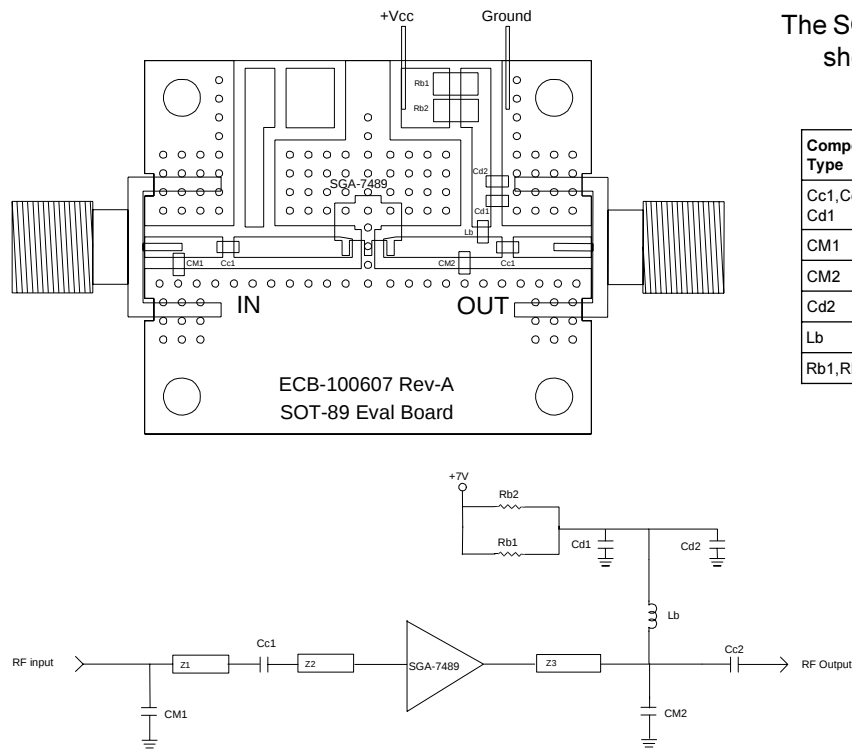
SGA-7489 2 GHz Application Circuit
