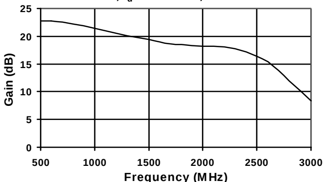
Gain vs. Frequency for 2GHz Tuned Circuit, I_d = 130 mA, T = +25^\circ\text{C}
