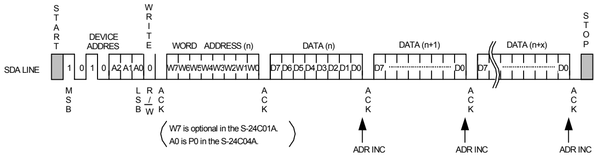
Figure 11 Page Write
