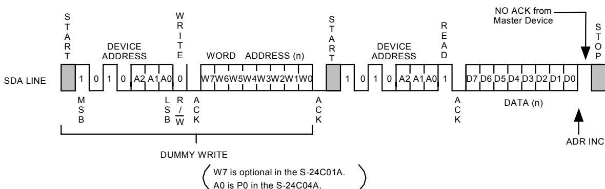
Figure 13 Random Read
