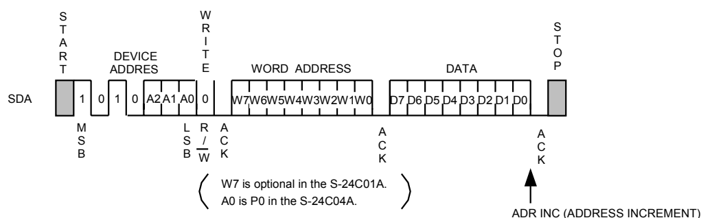
Figure 10 Byte Write
