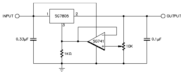
FIGURE 8 - ADJUSTABLE OUTPUT REGULATOR, 7V to 30V
