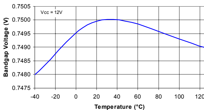
Bandgap Voltage vs Temperature
