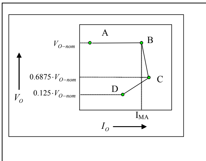
Figure 1. Over current protection characteristic of SC4602
