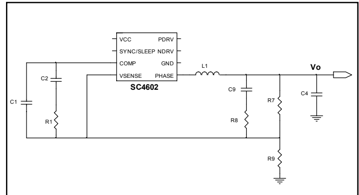
Figure 3. Compensation network provides 3 poles and 2 zeros.
