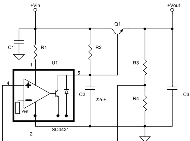
Linear Regulator Circuit
