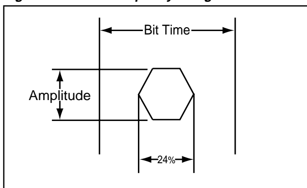
Figure 19. Receiver Input Eye Diagram Jitter Mask
