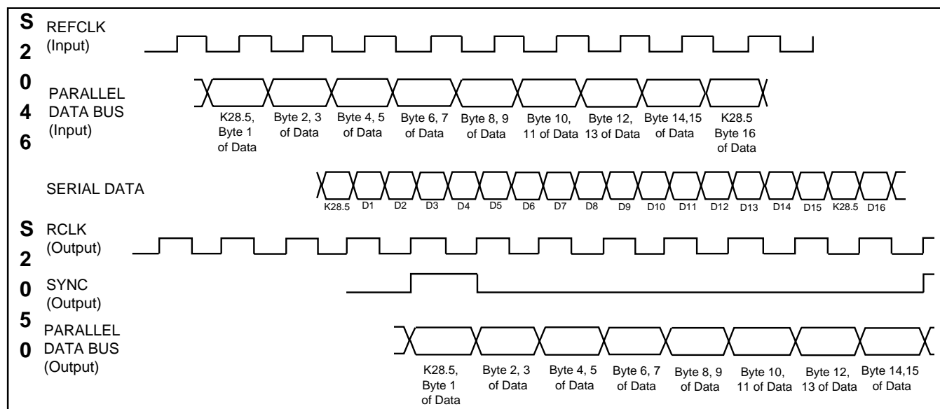
Figure 5. Functional Waveform
