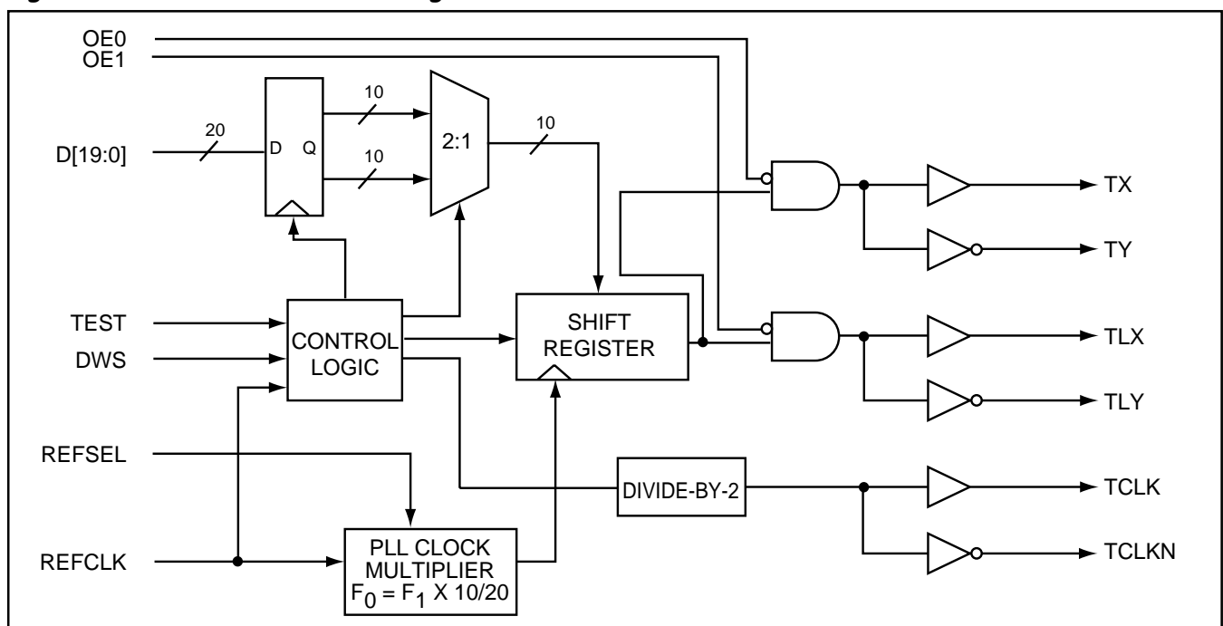
Figure 3. S2046 Functional Block Diagram
