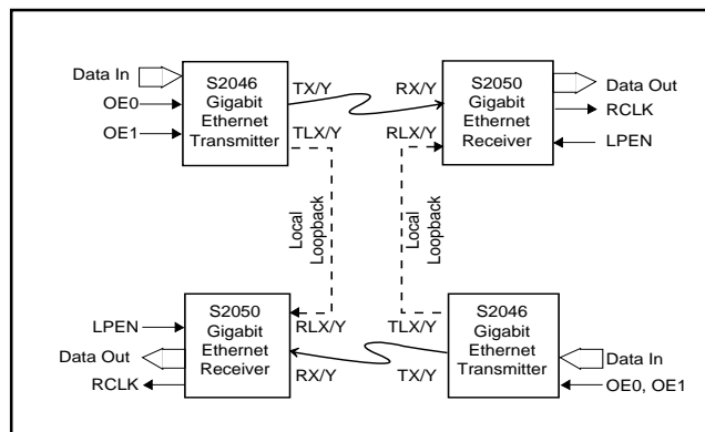
Figure 6. Interface Diagram
