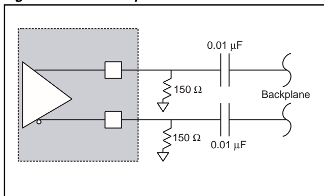
Figure 16. Serial Output Load
