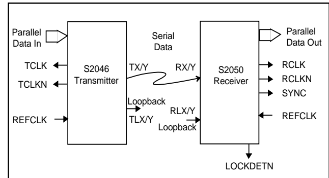
Figure 2. Interface Diagram
