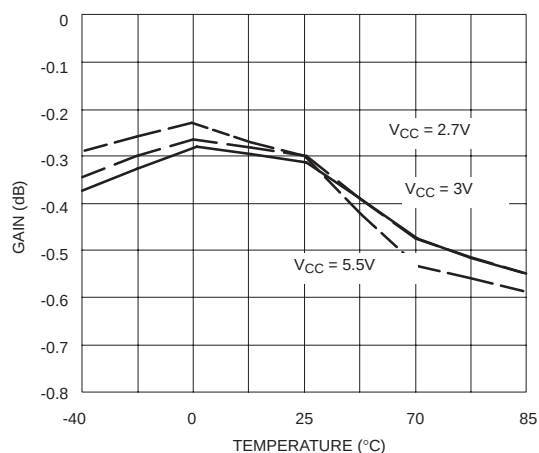
Post Detection Amplifier vs Temperature and V_{CC}
