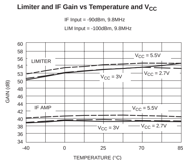
Figure 6. Typical Performance Characteristics
