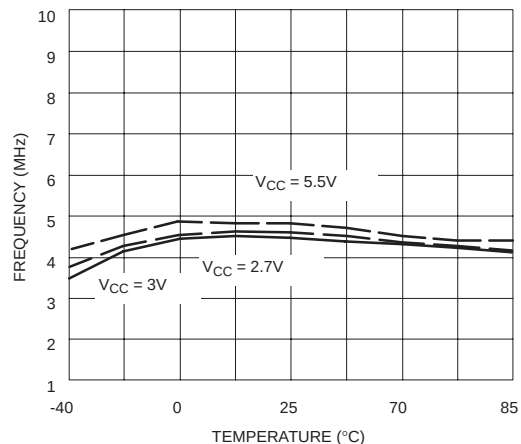
Post Detection Amplifier -3dB Bandwidth vs Temperature and V_{CC}
