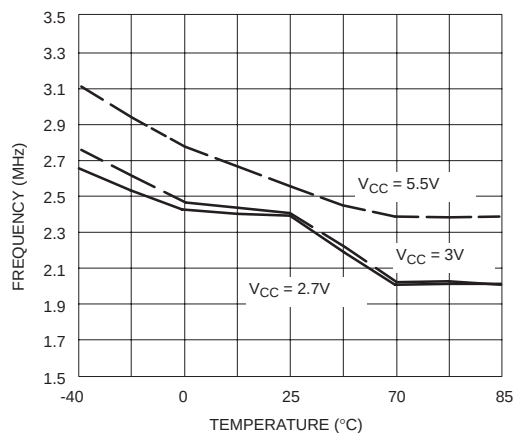
Data Output -3dB Bandwidth vs Temperature and V_{CC}
