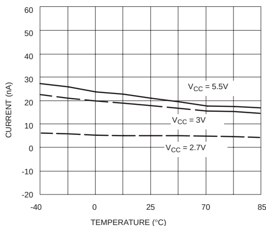
Figure 8. Typical Performance Characteristics (cont.)
