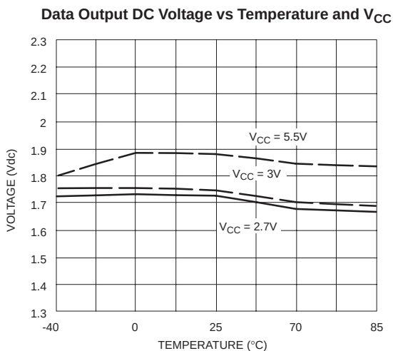
Figure 7. Typical Performance Characteristics (cont.)
