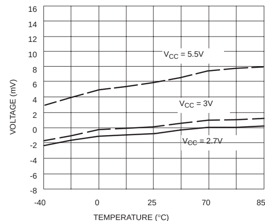
Switch Output to Input Offset Voltage vs Temperature and V_{CC}
