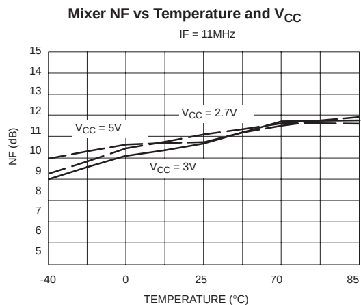
Figure 6. Typical Performance Characteristics
