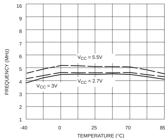
Post Detection Amplifier -3dB Bandwidth vs Temperature and V_{CC}
