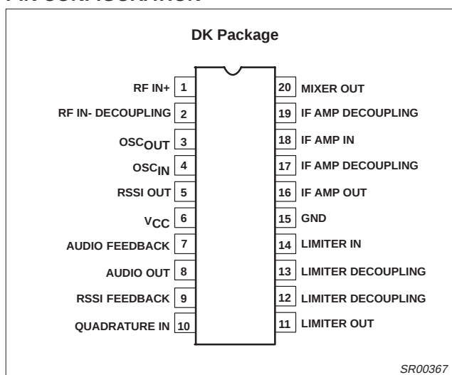
Figure 1. Pin Configuration
