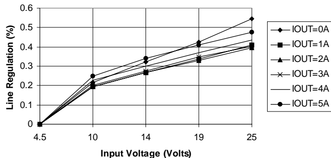
SC1480EVb Line Regulation at V_{out} = 1.25V
