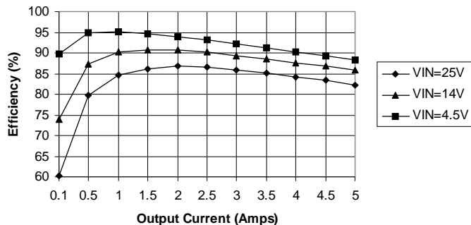
SC1480EVb Efficiency at V_{out} = 1.25V
