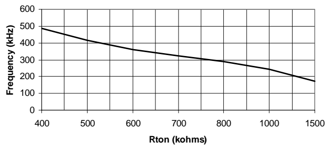
R_{ton} vs Frequency ( V_{in} = 15V , V_{out} = 1.25V , I_{out} = 1A )
