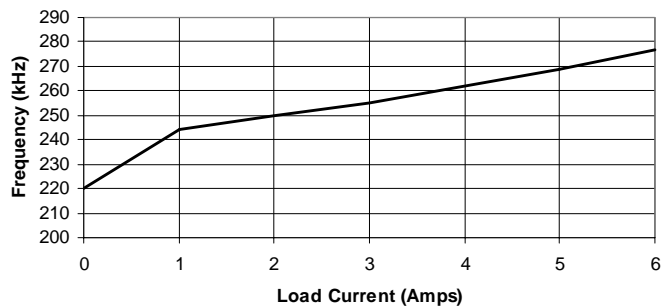
Frequency vs Load Current ( V_{in} = 15V , V_{out} = 1.25V , R_{ton} = 1M )
