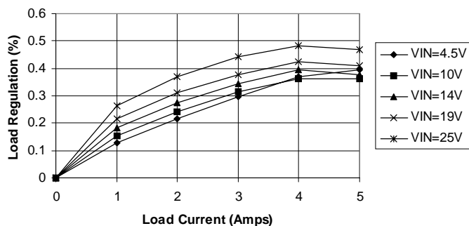
SC1480EVb Load Regulation at V_{out} = 1.25V
