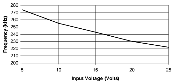
Frequency vs Input Voltage ( I_{out} = 1A , V_{out} = 1.25V , R_{ton} = 1M )
