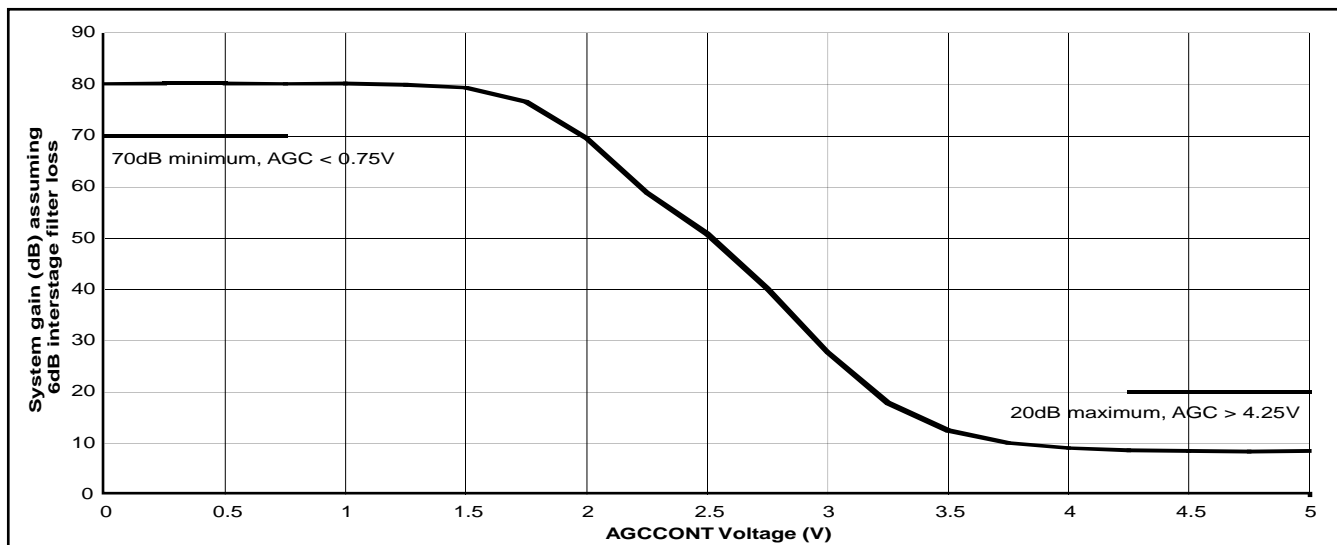
Figure 4. AGC characteristic (typical)
