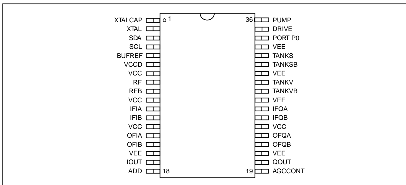
Figure1. Pin connections
