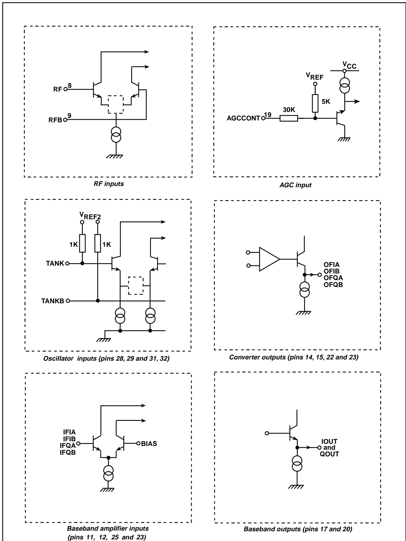
Figure 17. Input and output interface circuits (RF section)
