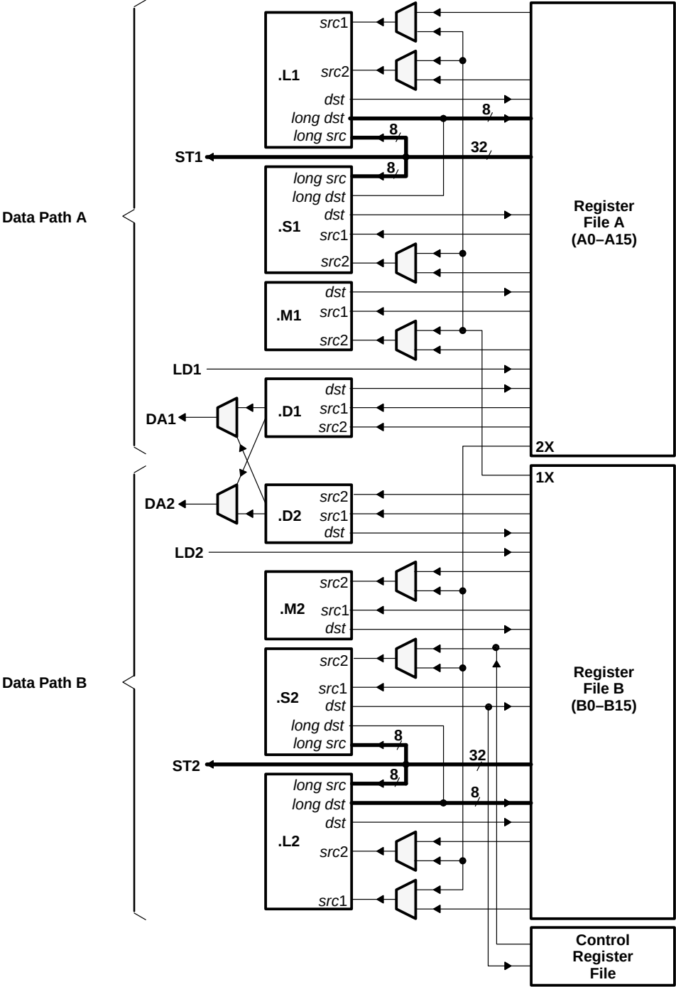
Figure 1. SM320C62x CPU (DSP Core) Data Paths
