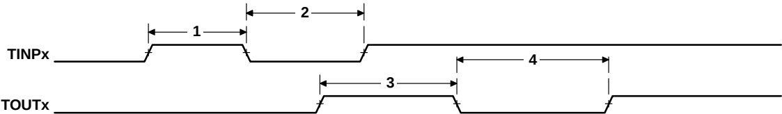
Figure 54. Timer Timing
