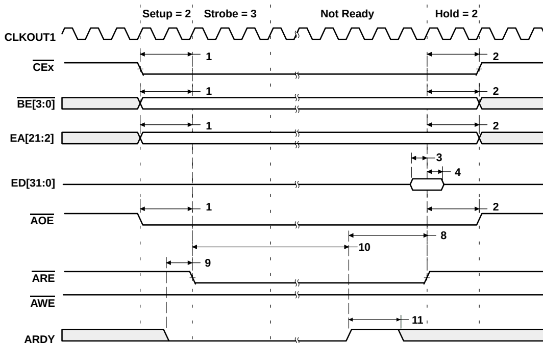
Figure 17. Asynchronous Memory Read Timing (ARDY Used)
