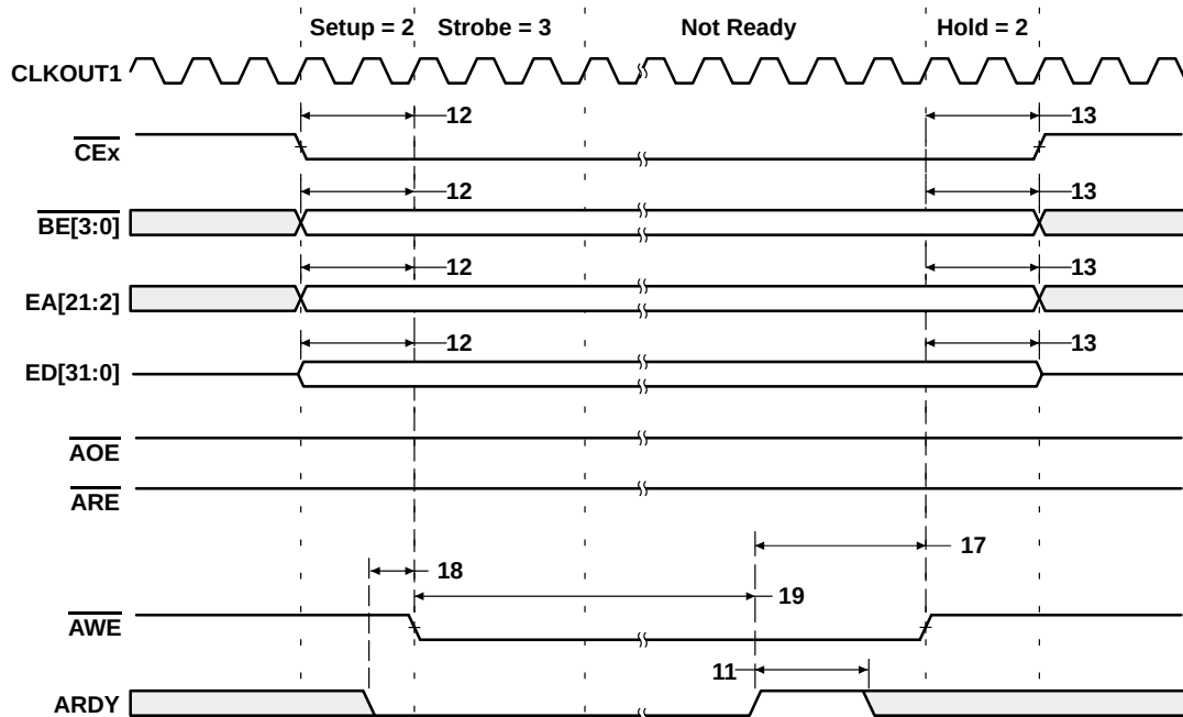
Figure 19. Asynchronous Memory Write Timing (ARDY Used)
