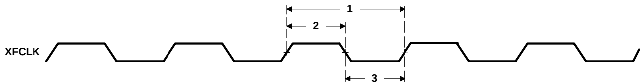
Figure 15. XFCLK Timings
