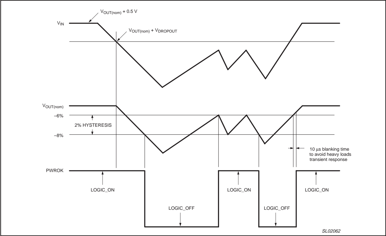
Figure 8. Timing diagram.
