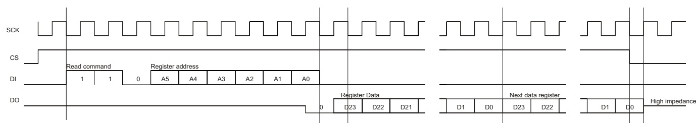
Figure 5: SPI waveforms
