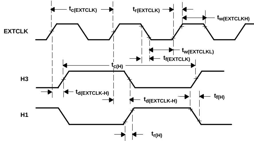
Figure 17. Divide-By-Two Mode
