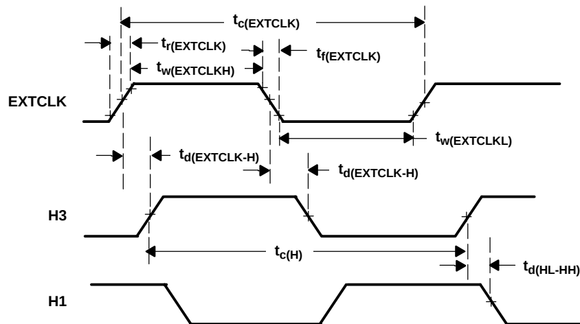
Figure 17. Divide-By-Two Mode
