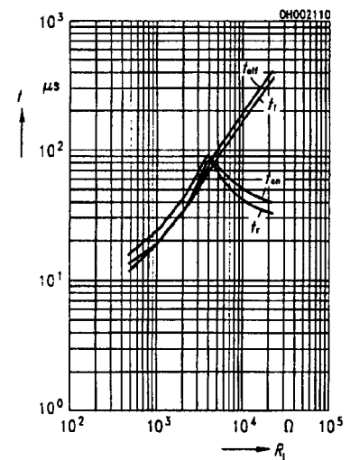
Figure 2. Switching Times T_A=25^\circ\text{C} , I_F=1.0\text{ mA} , V_{CC}=5.0\text{ V} , t_{ON} , t_R , t_{OFF} , t_F , =f(R_L)
