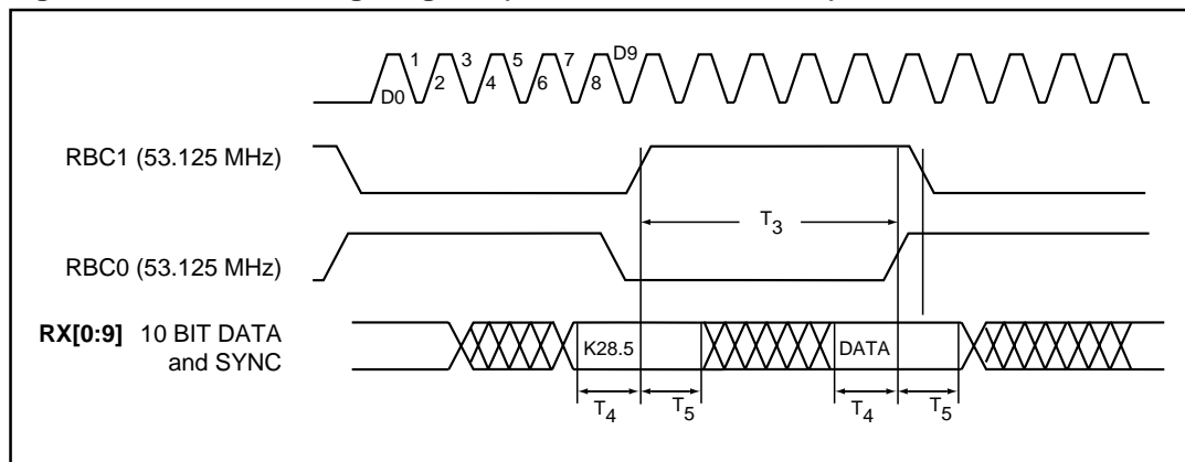
Figure 8. Receiver Timing Diagram (1062.5 Mbits/sec mode)
