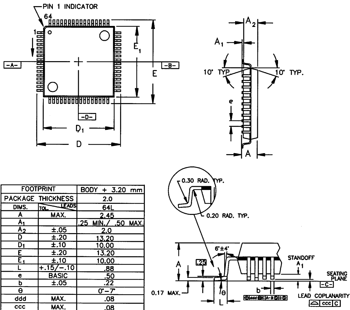
Figure 5. 64 PQFP (10mm x 10mm) Package
