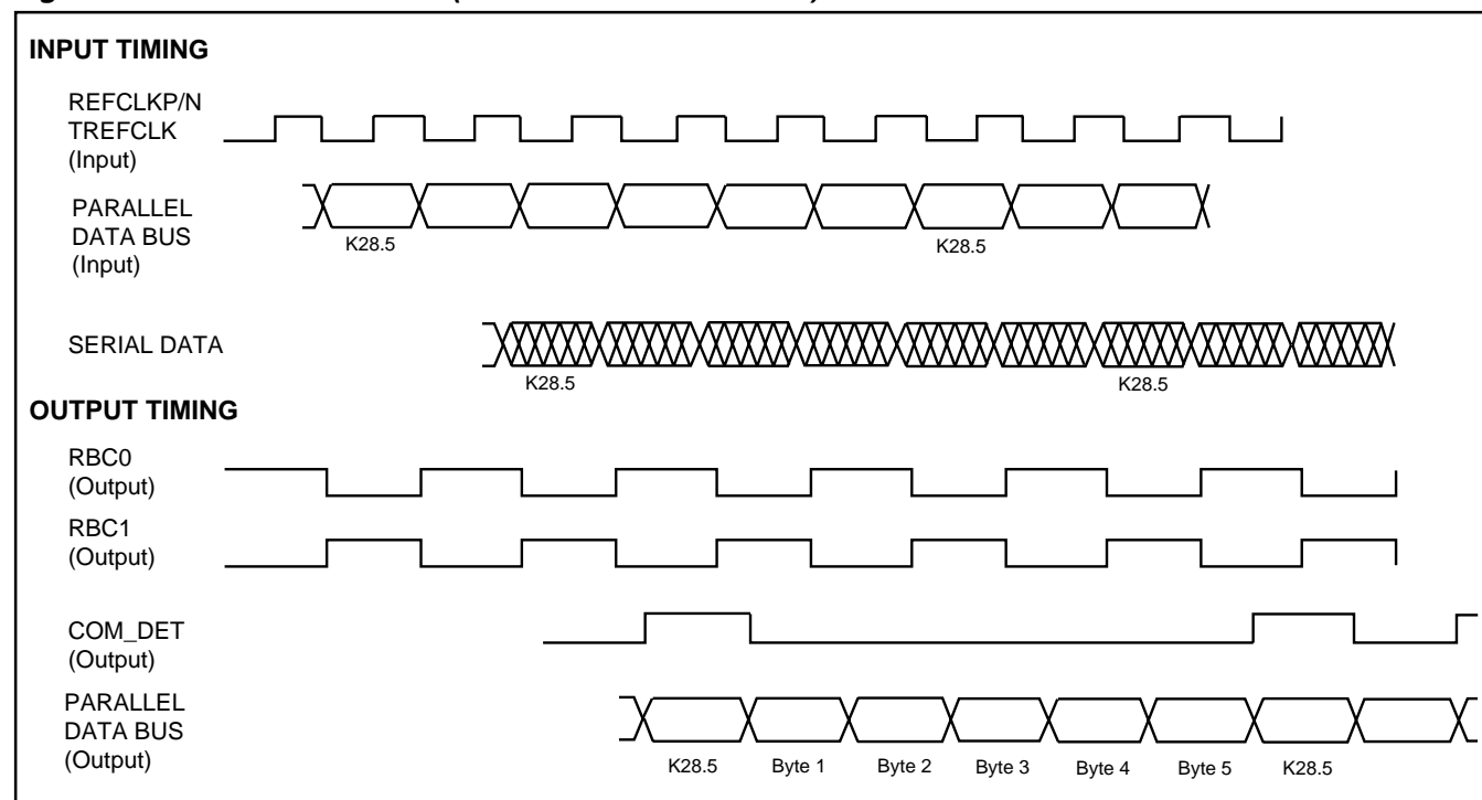
Figure 4. Functional Waveform (1250 and 1062.5 Mbit/sec)
