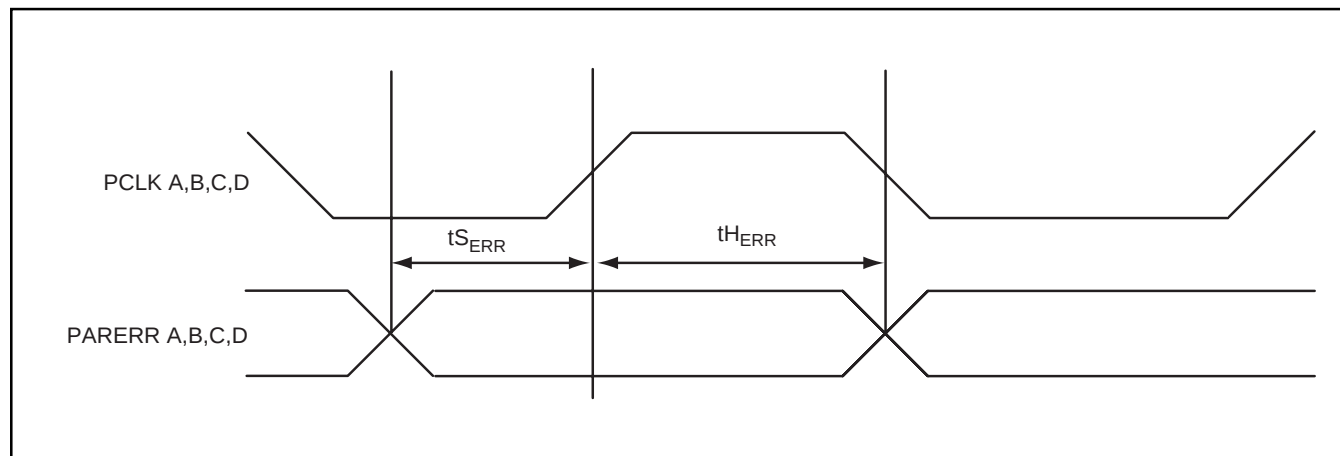
Figure 17. AC Parity Error Timing Diagram
