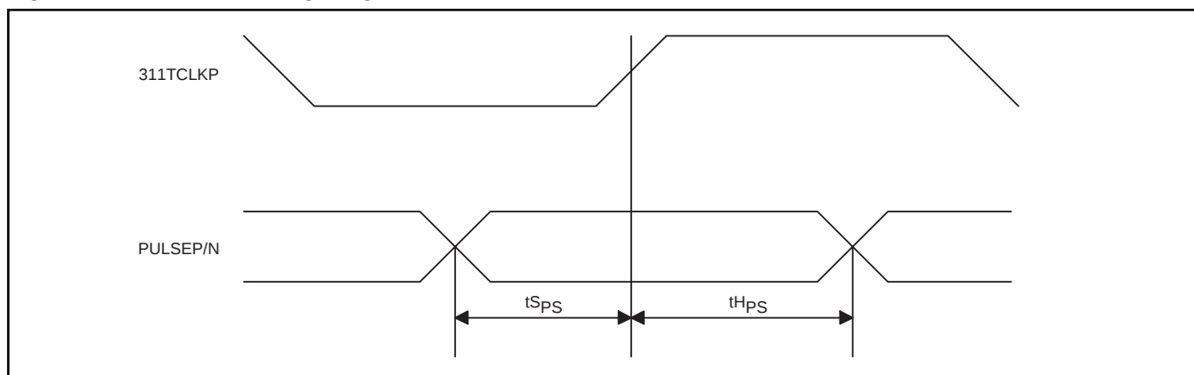
Figure 20. AC Pulse Timing Diagram
