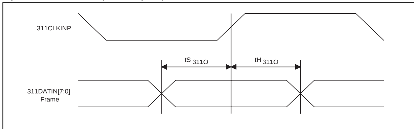
Figure 19. AC Receiver Input Timing Diagram
