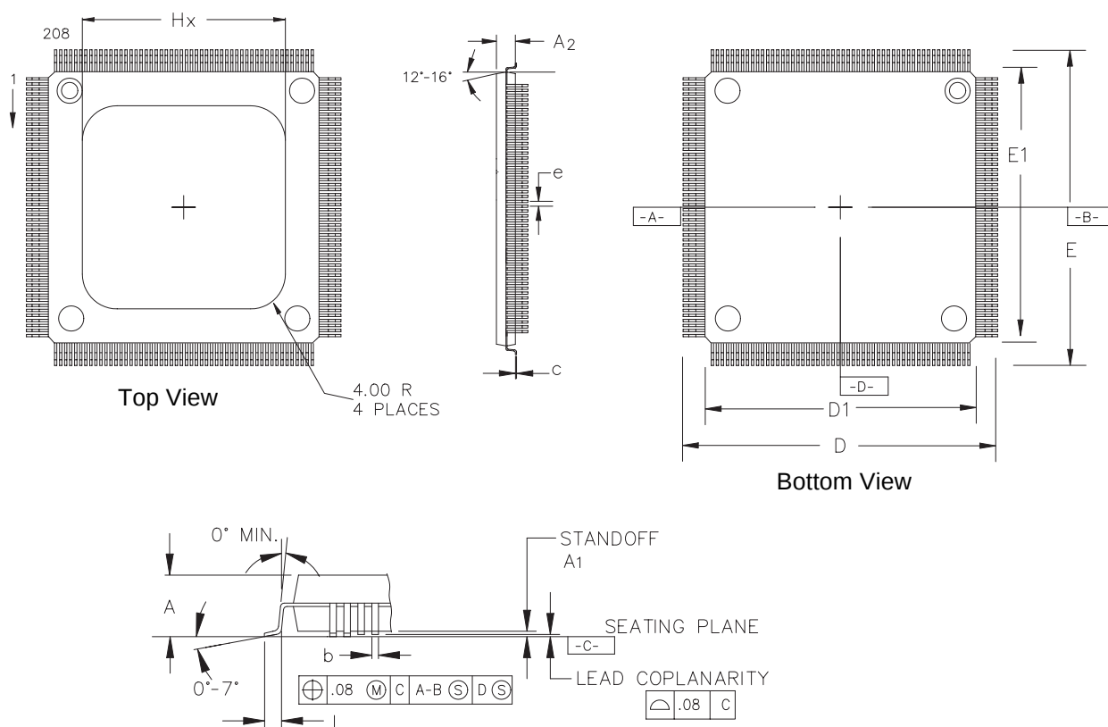
Figure 15. S3045 208 PQFP TEP (28 x 28 x 3.40mm) - Plastic Quad Flat Pack
