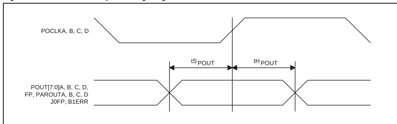
Figure 21. AC Receiver Output Timing Diagram
