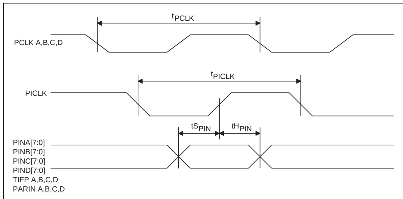
Figure 16. AC Transmitter Parallel Input Data Timing Diagram
