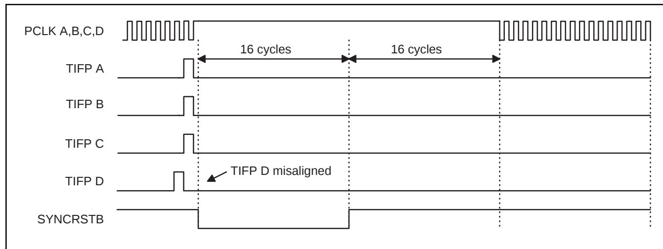
Figure 3. S3045 Synchronous Reset Functional Timing Diagram
