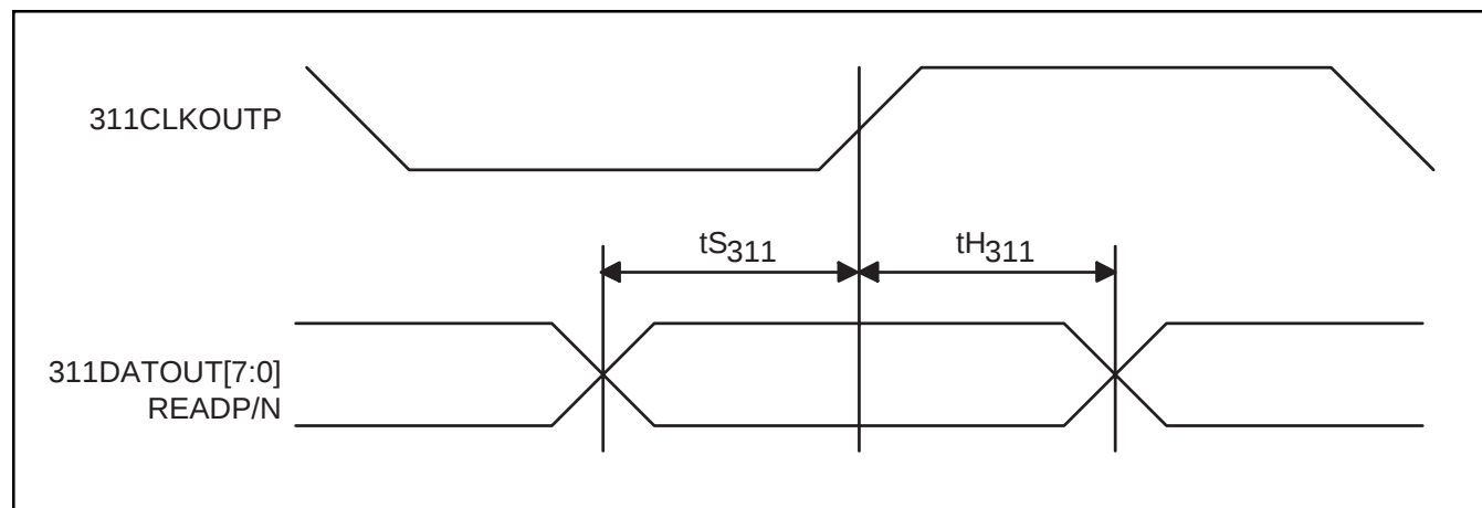
Figure 18. AC Transmitter Output Timing Diagram
