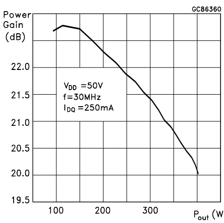
Power Gain vs Output Power
