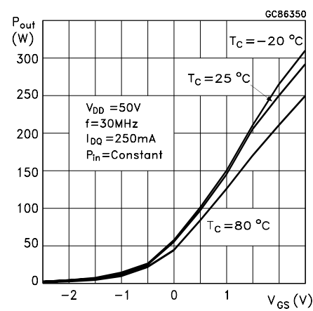
Output Power vs Gate Voltage
