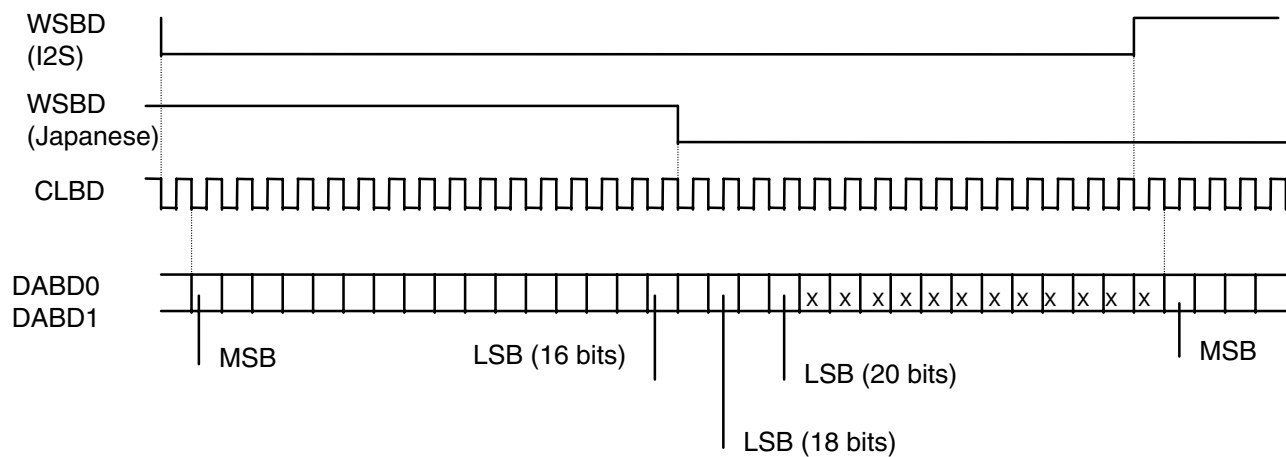
Figure 4. Digital Audio Frame Format (1)
