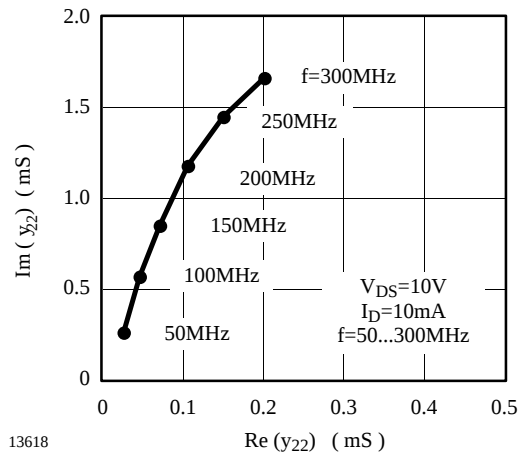
Figure 8. Short Circuit Output Admittance
