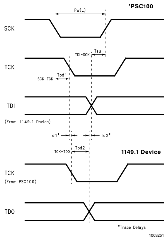
FIGURE 16. System Clock Timing for Accurate TDI Data
