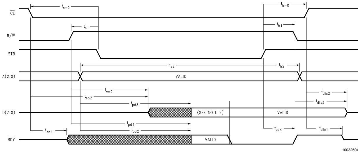
FIGURE 3. Read Cycle
