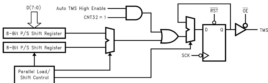
FIGURE 10. TMS Shifter/Buffer Block Diagram
