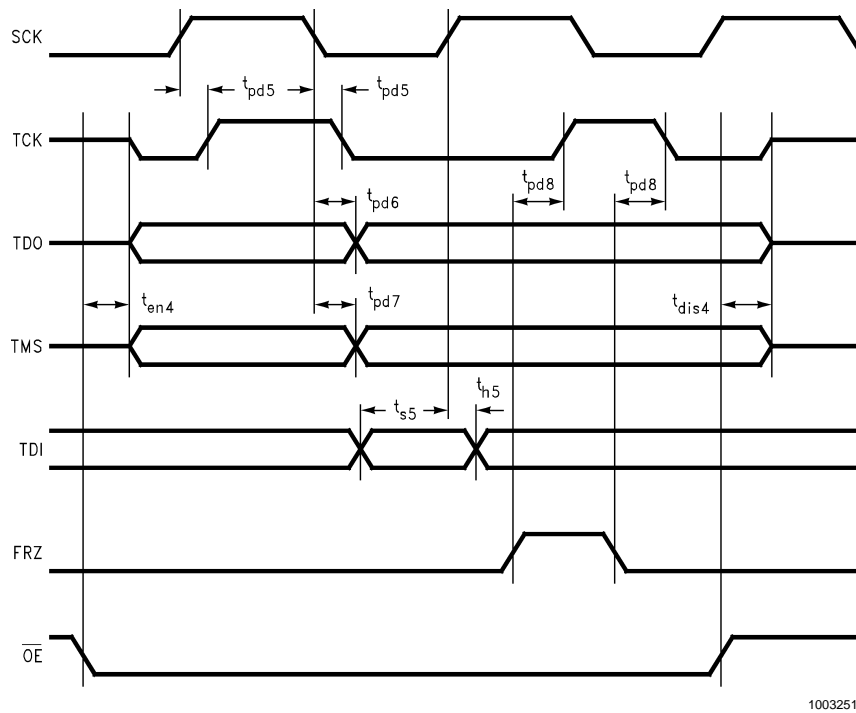
FIGURE 15. Serial Scan Interface Timing
