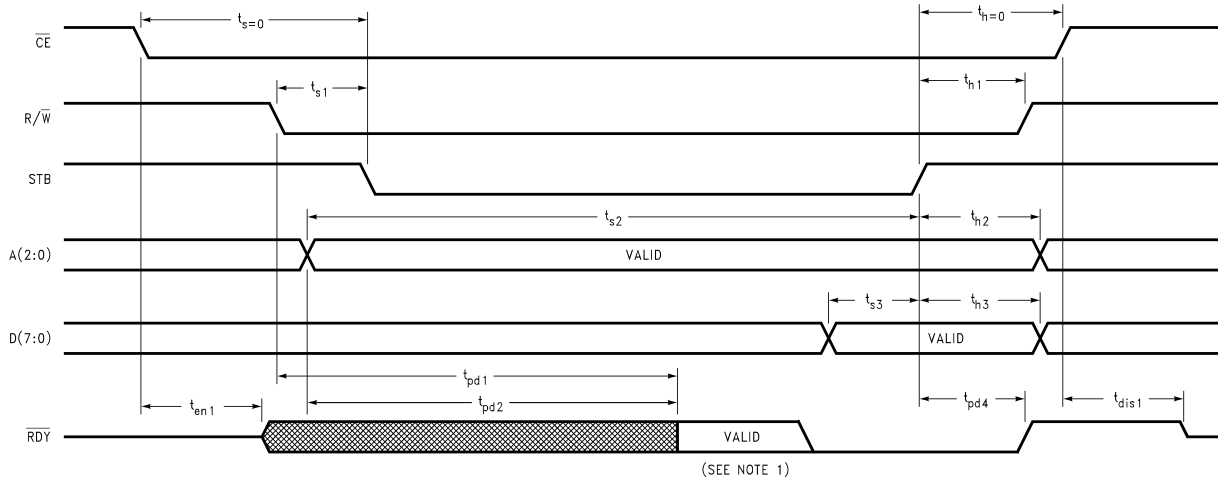
FIGURE 2. Write Cycle
