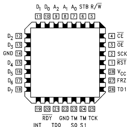
Pin Assignment for LCC
