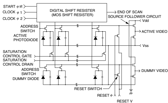
Figure 1 Equivalent circuit
