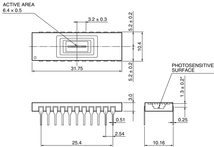
Figure 3 Dimensional outlines (unit: mm)
