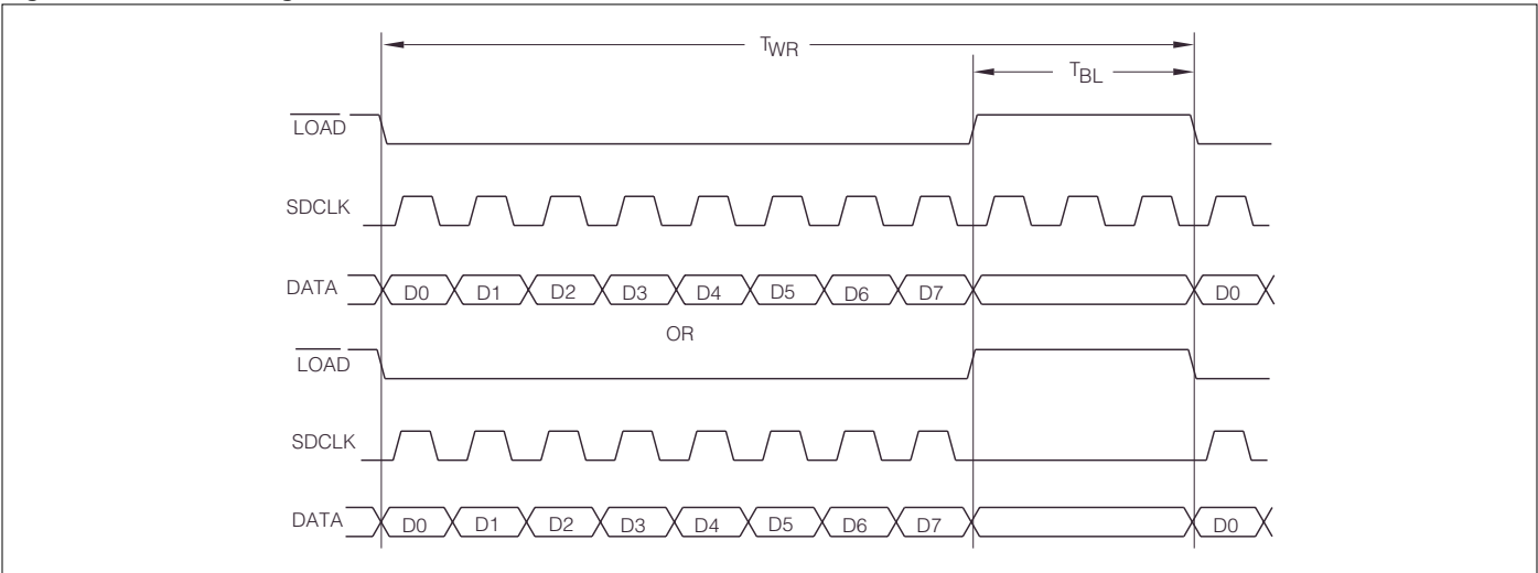
Figure 3. Device Timing
