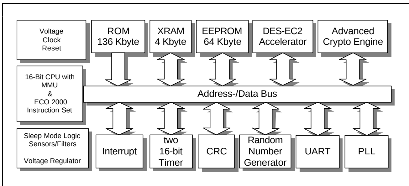
Figure 2: Block Diagram SLE 66CX640P
