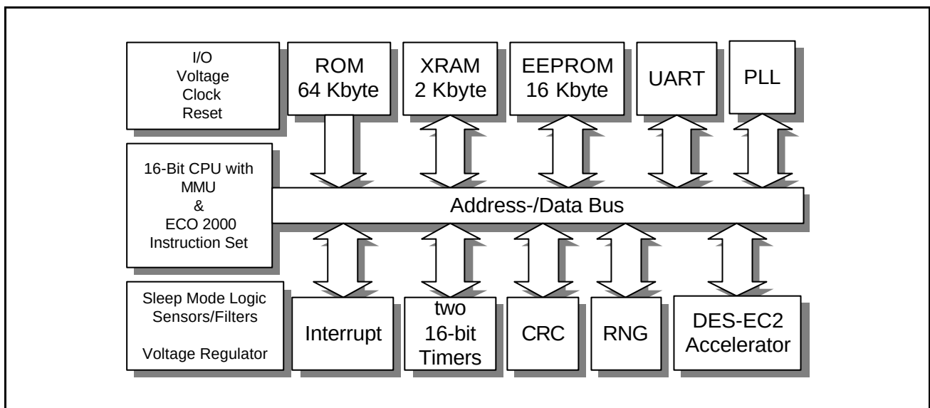
Figure 2: Block Diagram SLE 66C160P
