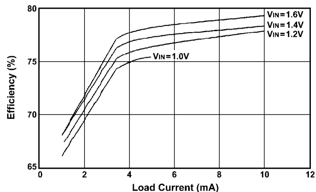
Figure 4. 1-Cell Input 5V Output Step-Up Converter
