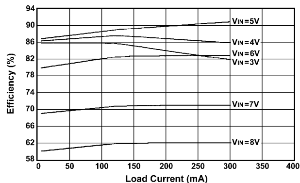
Figure 5. 4-Cell Input Step-Up/Step-Down Converter
