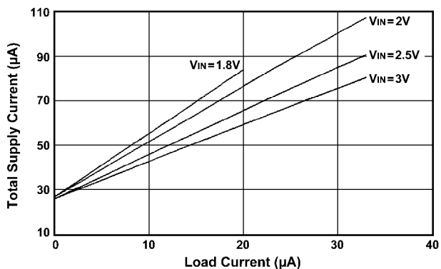
Figure 6. Low Supply Current Burst Mode Step-Up Converter
