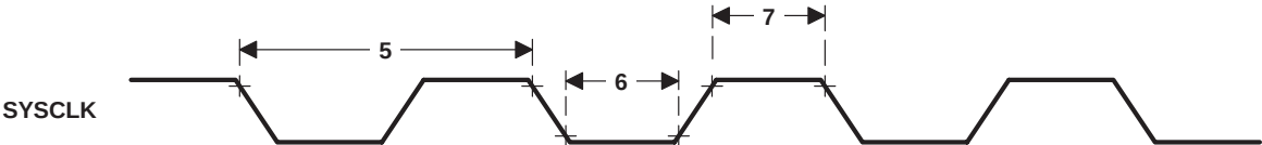
Figure 25. SYSCLK Timing
