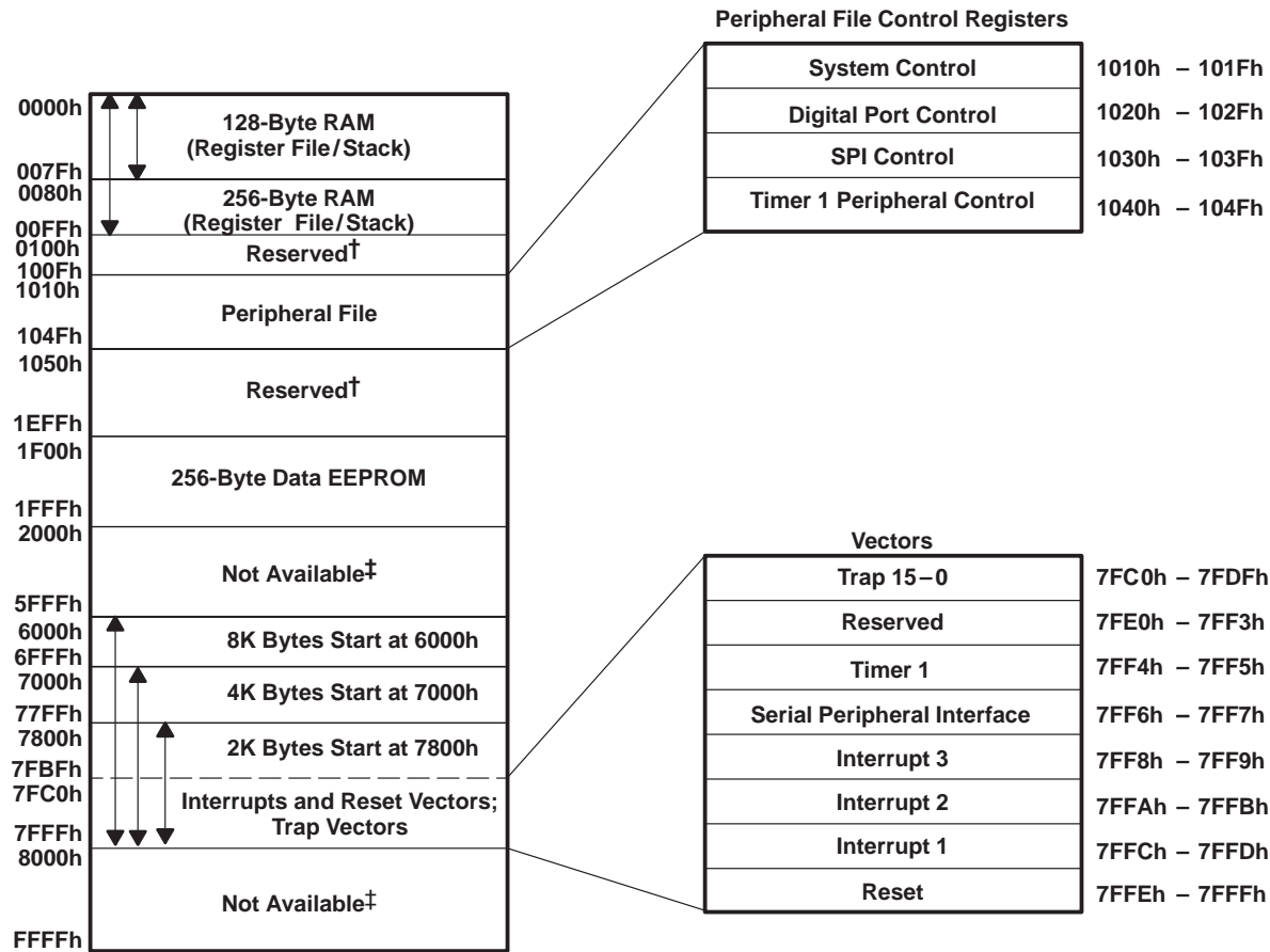
Figure 3. TMS370Cx1x Memory Map
