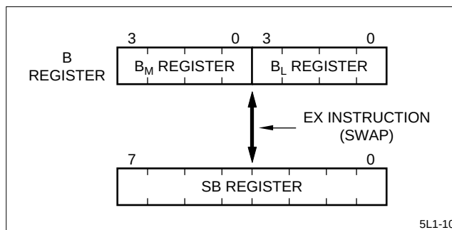
Figure 10. B Register and SB Register
