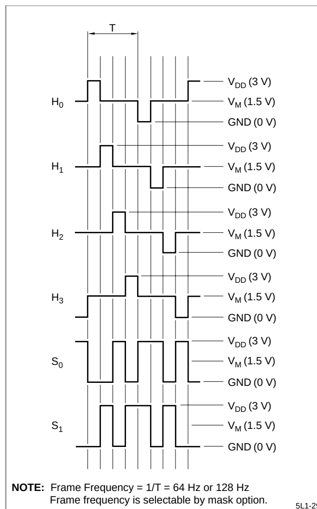
Figure 29. LCD Drive Waveforms
