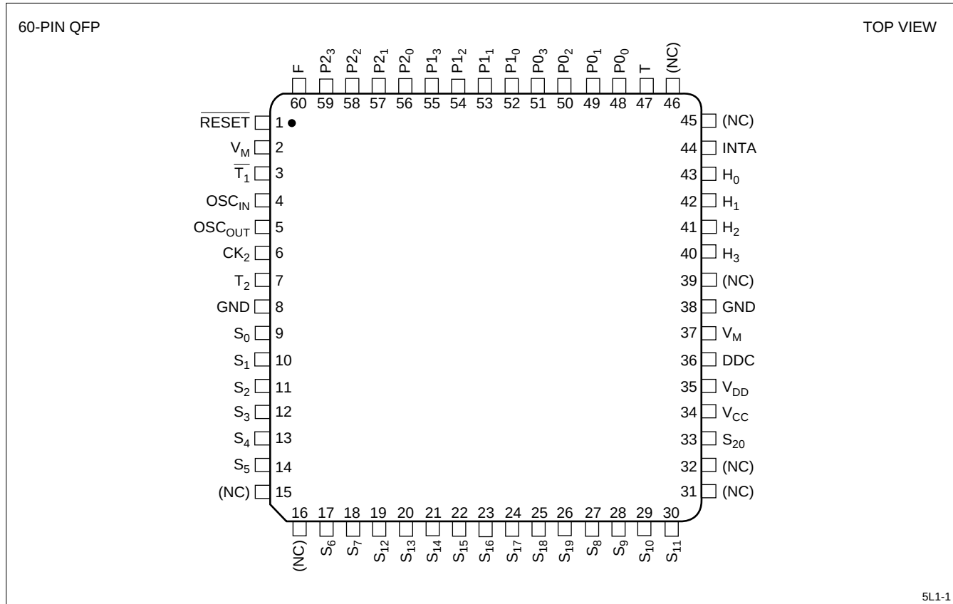
Figure 1. 60-pin QFP (SM5L1)
