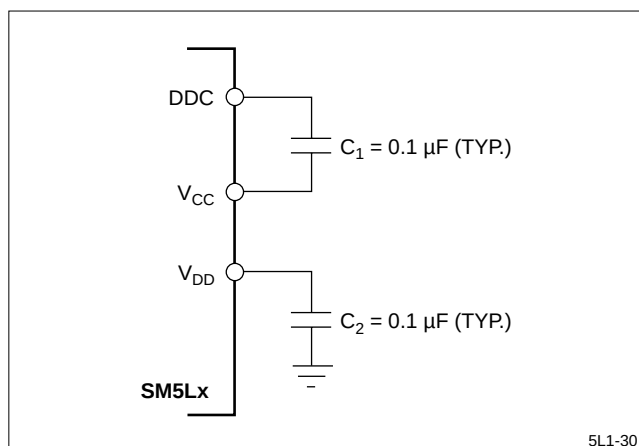
Figure 30. Booster Circuit
