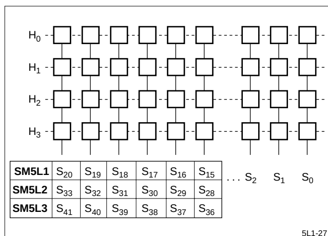
Figure 27. LCD Pattern
