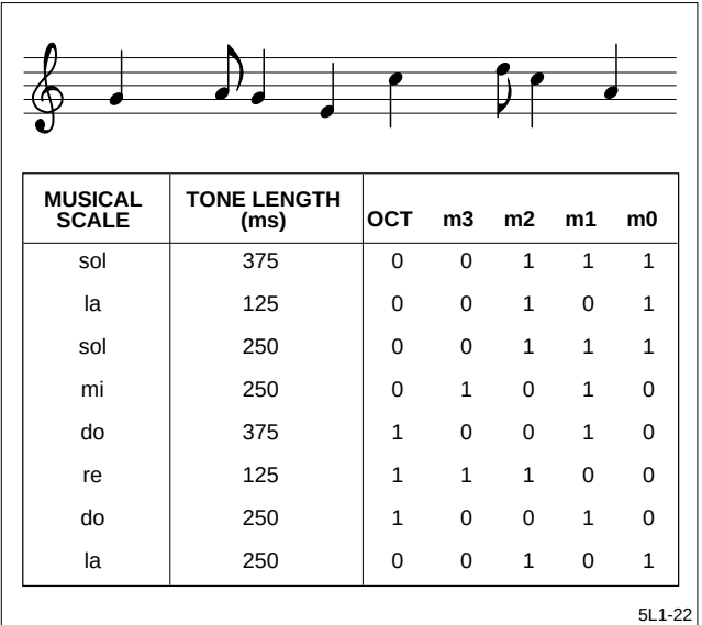
Figure 22. Melody ROM Tone Writing Example
