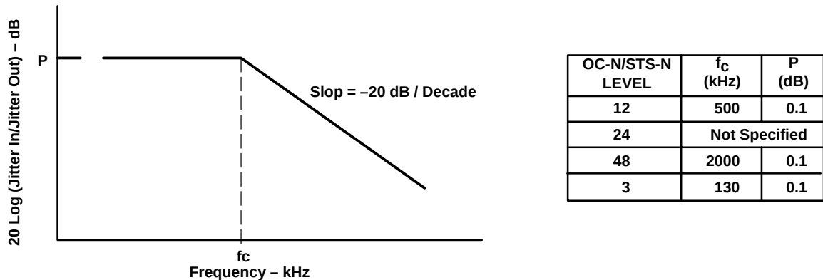
Figure 2. Jitter Transfer
