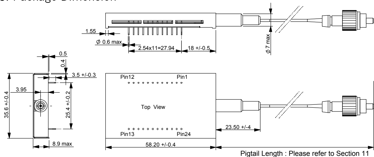
Figure 2 Package Dimension
