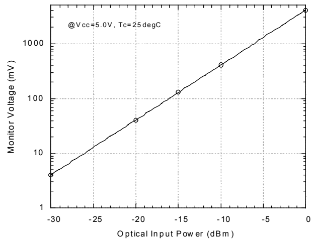
Figure 5 Relation Between Optical Input Power
