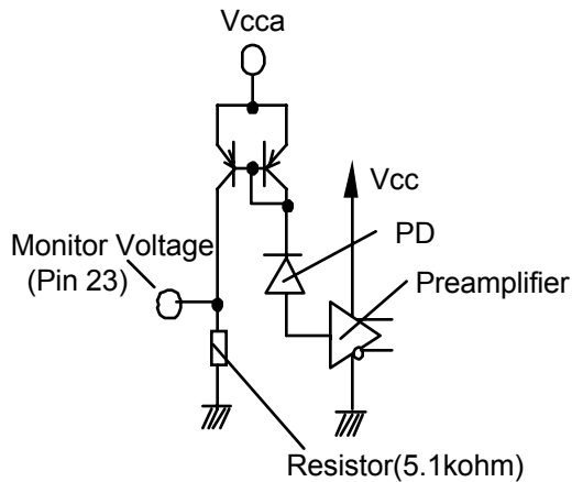
Figure 4 Input Power Monitoring Circuit
